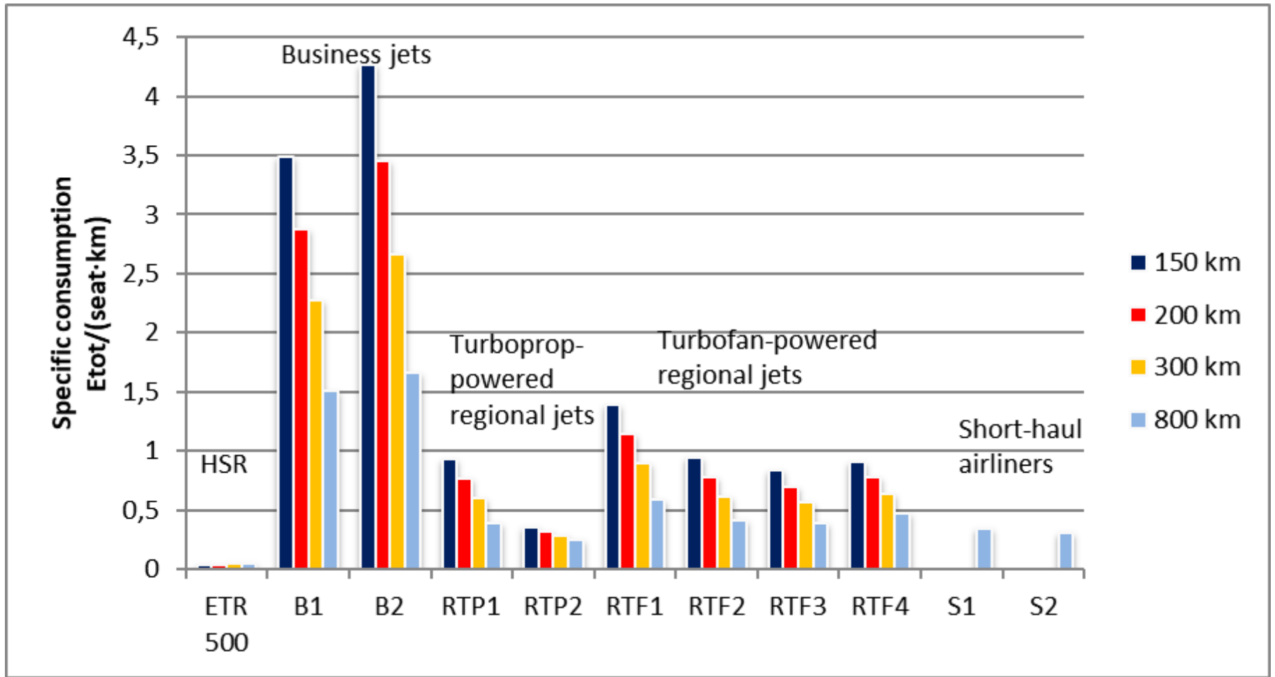
Comparison of the specific consumption (kWh /pax-km) of HSR and of air transport
